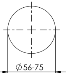
Mounting Hole
