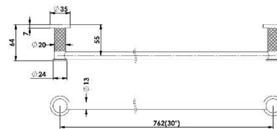
762mm DOUBLE TOWEL RAIL
