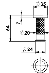
DOUBLE ROBE HOOK
