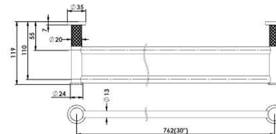
762mm DOUBLE TOWEL RAIL
