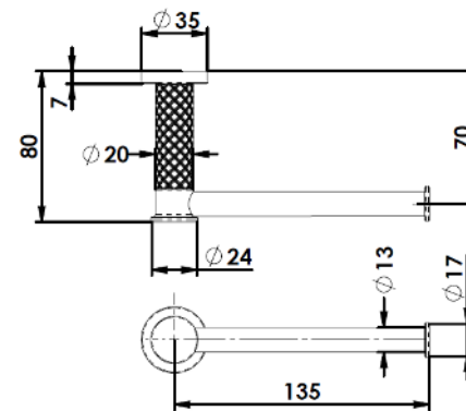
762mm SINGLE TOWEL RAIL
