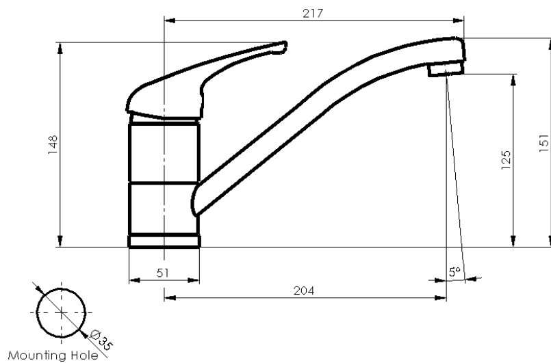
Sink Mixer
